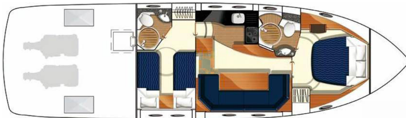
Lower deck
