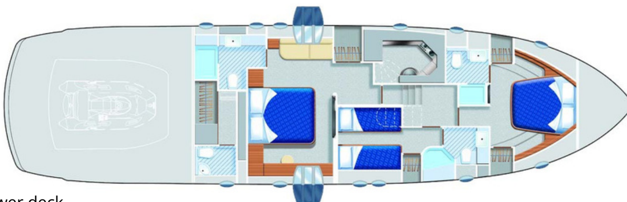
Lower deck
